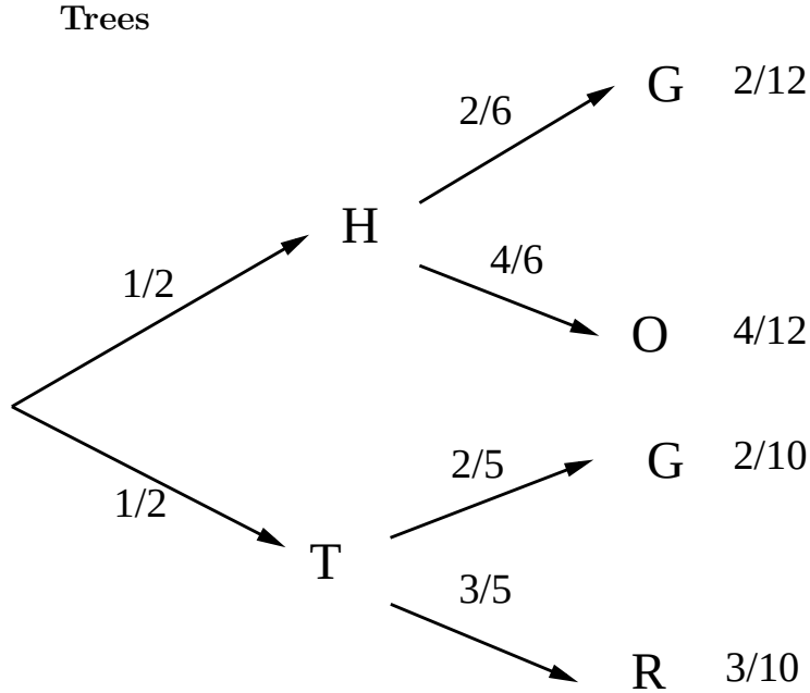
Figure 1: Tree for the example with flipping a coin and then removing some balls from the urn.
