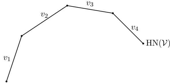
FIGURE 1. Vector representation of \text{HN}(\mathcal{V}) .
